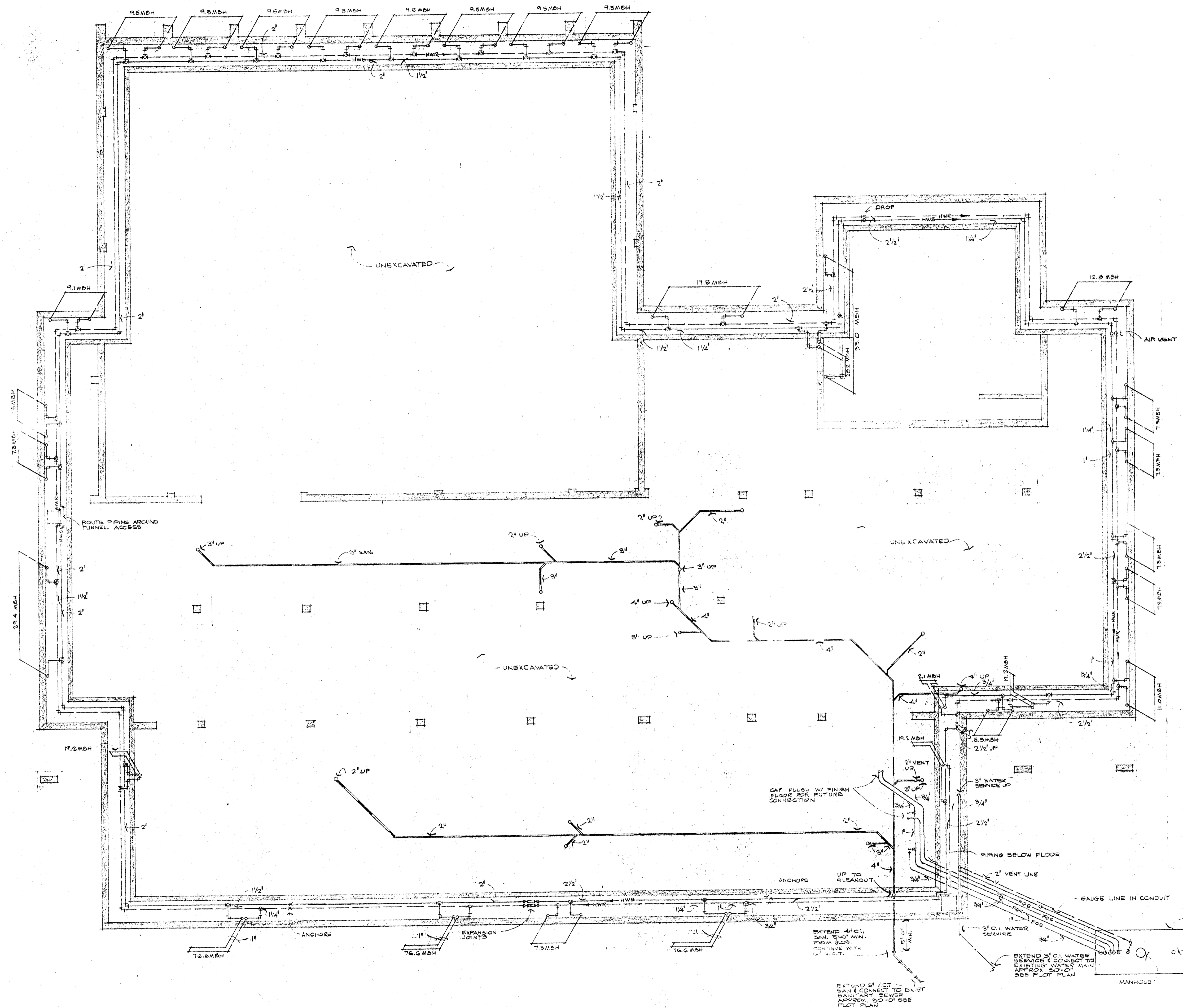
① FOUNDATION PLAN — LIBRARY SCALE 1/8" = 1'-0"
