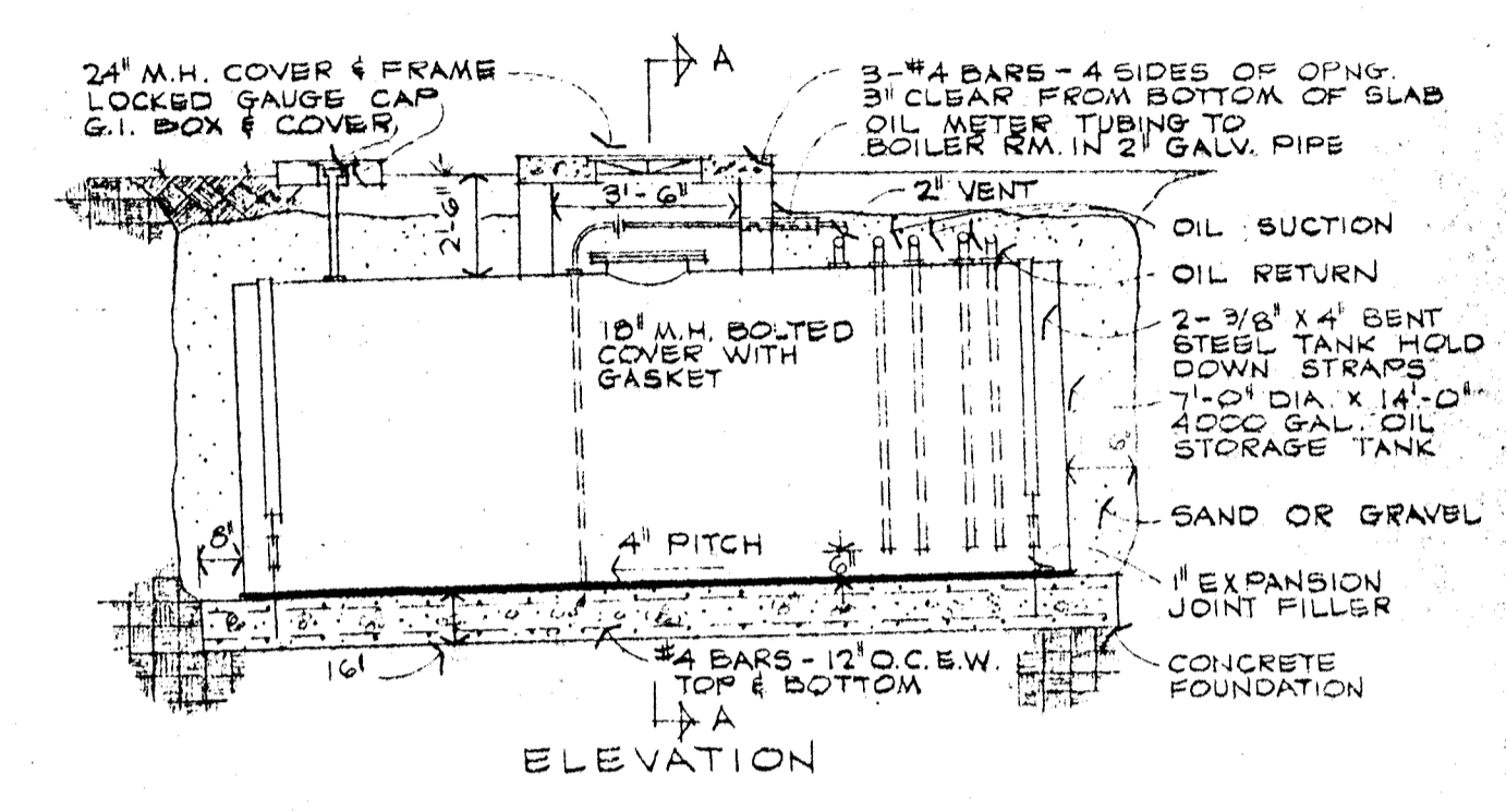
② OIL STORAGE TANK DETAIL NO SCALE M-4
